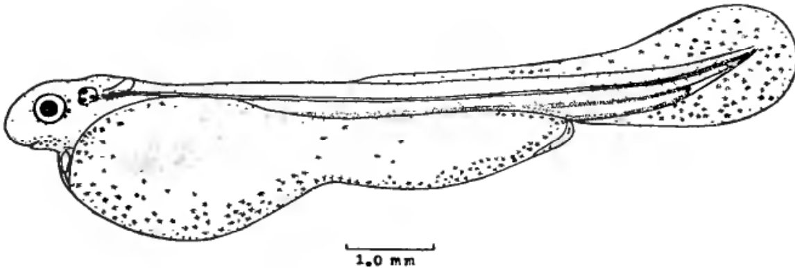
Fig. 1. First day hatching of T. tor (Ham.)
